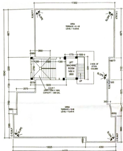
ROOF PLAN SCALE = 1:100
